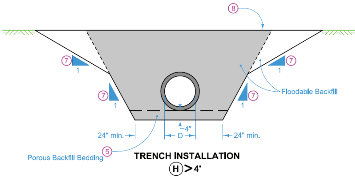
Figure 8-4: Trench installation with no flowable mortar cap.
