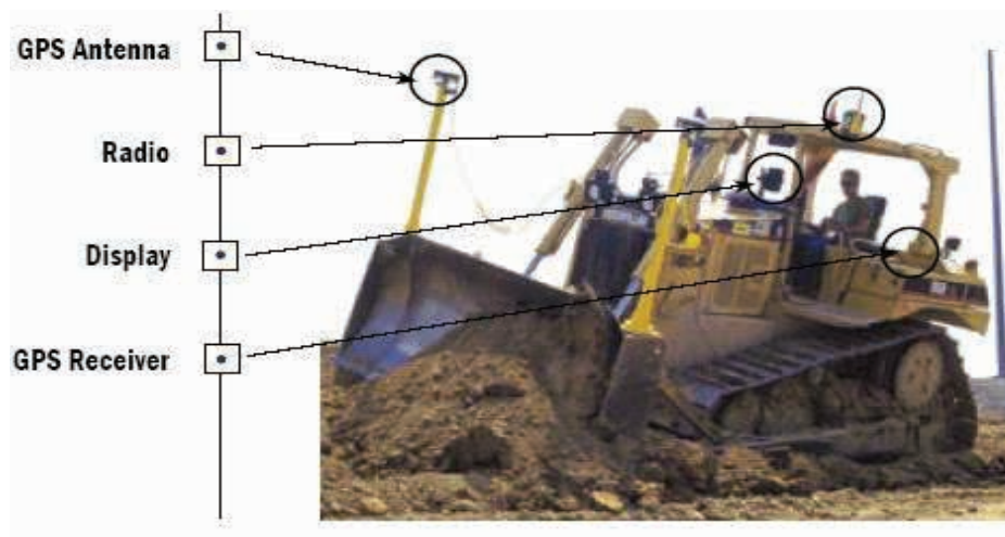
Figure 4-12: Dozer equipped with GPS.
