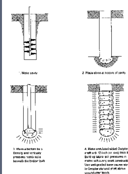
Figure 6.3.1. Geopier Construction 4-Step Process
