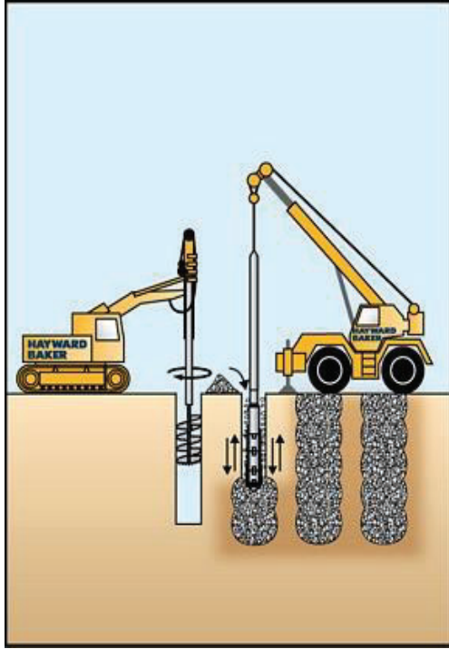
Figure 9-10: Illustration and photo showing installation of stone columns
