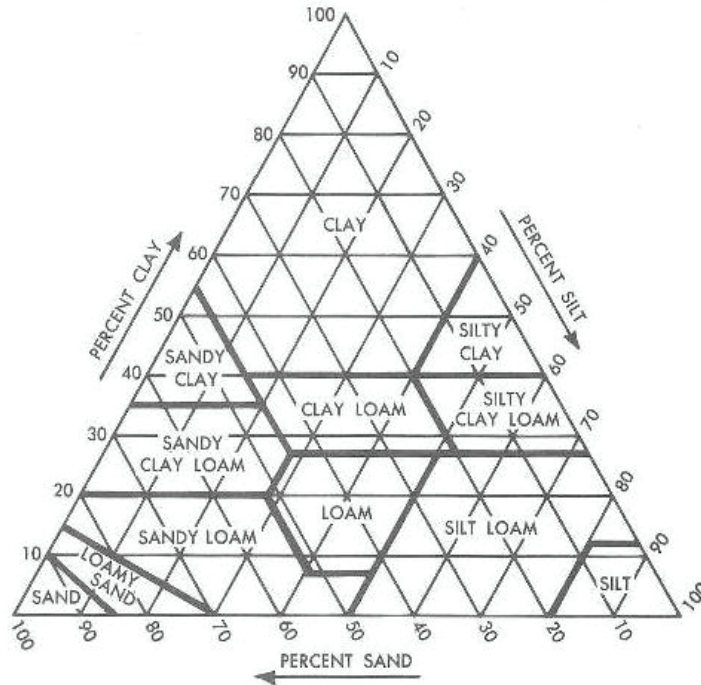
Figure 2-7: USDA textural classification triangle.
