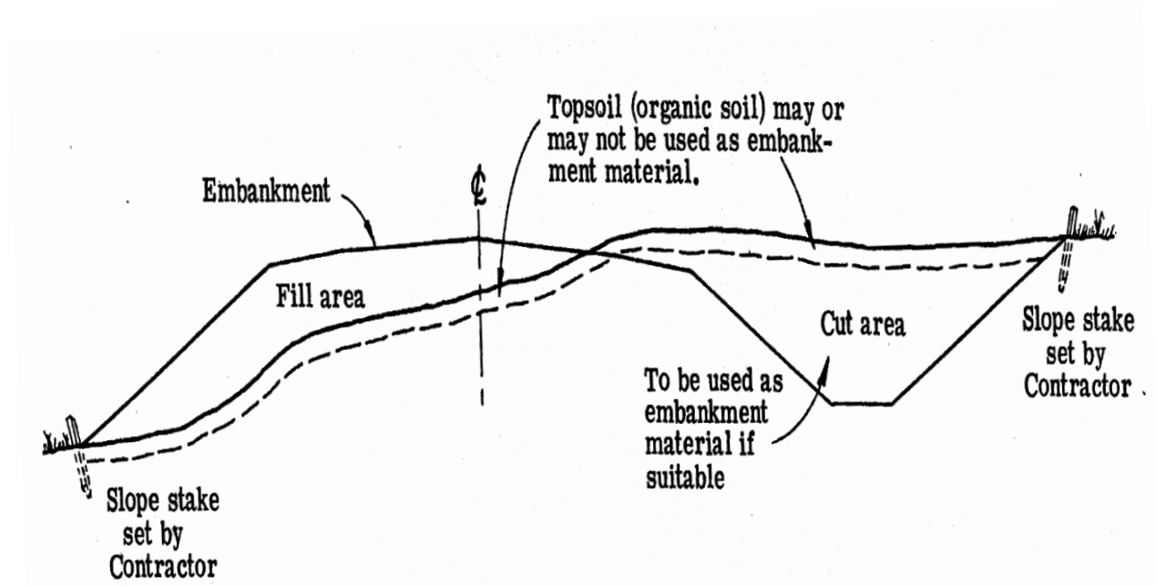
Figure 6-1: Cut and fill areas showing excavation and embankment construction.
