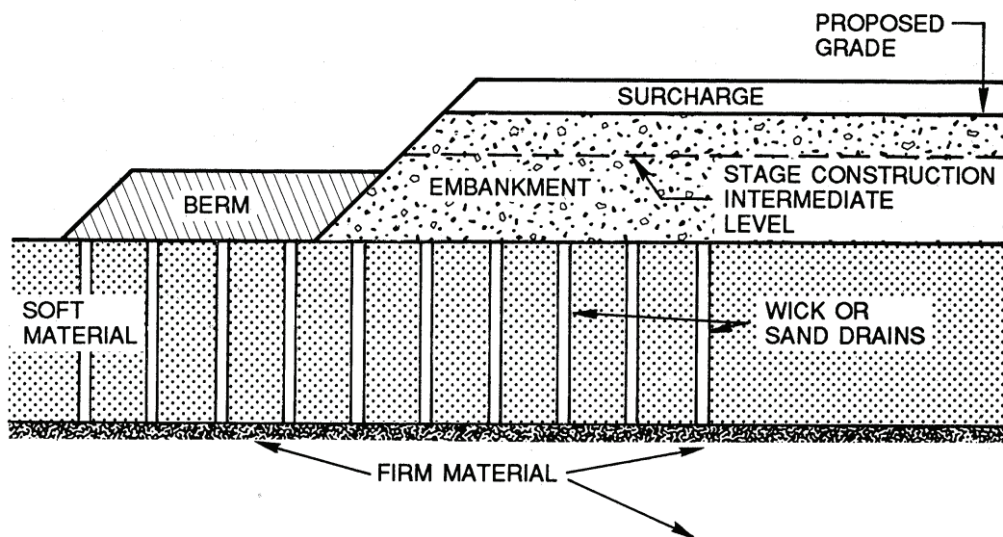
Figure 9-7: Illustration of wick or sand drains used to accelerate consolidation of soft material
