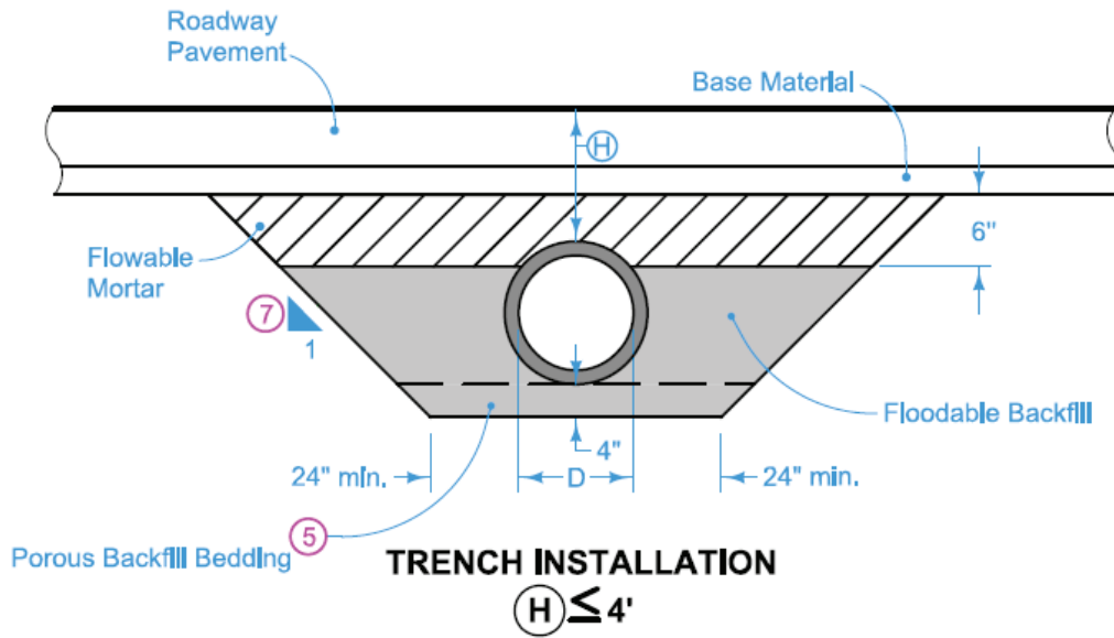
Figure 8-3: Shallow trench installation with flowable mortar cap.
