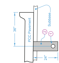
TYPE 12 INSTALLATION SECTION D-D
