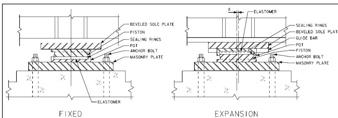
Figure 4.3.2-5 Pot Bearings
