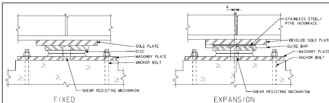
Figure 4.3.2-4 Disc Bearings
