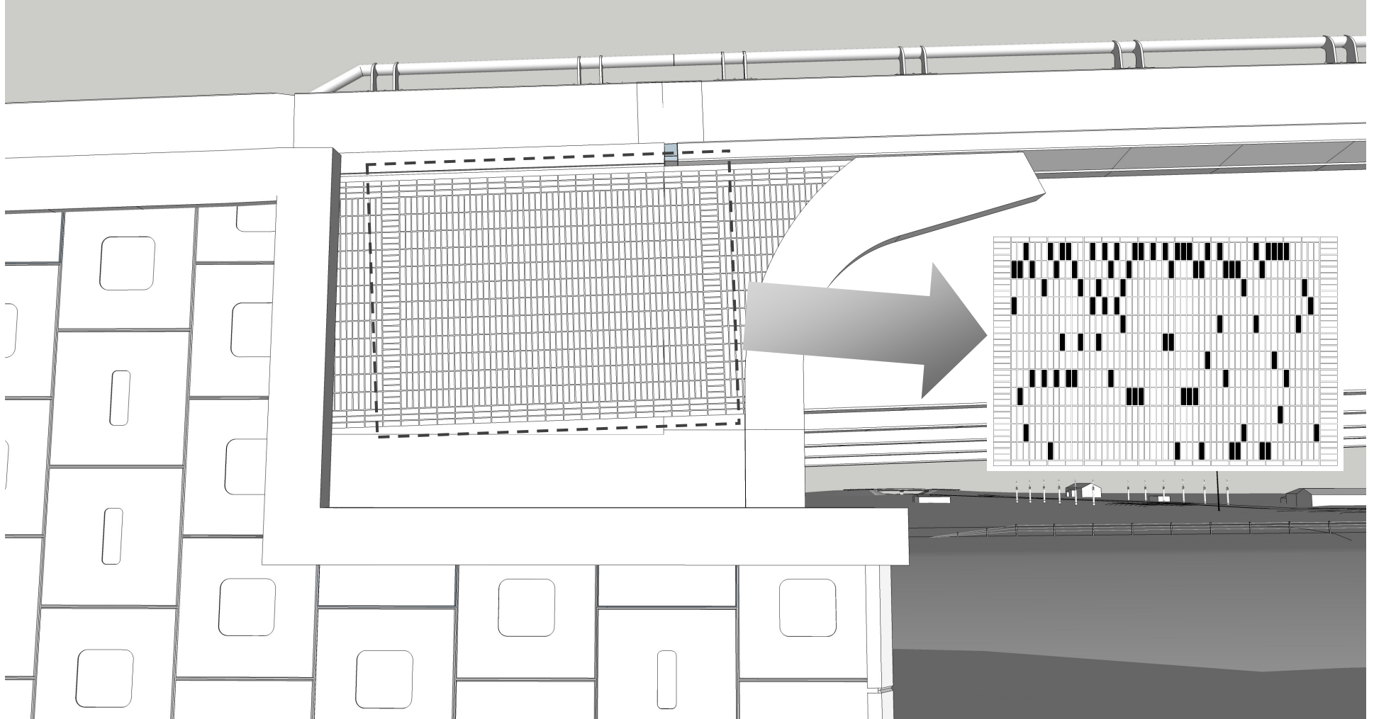
Abutment "Card Section" Typical Location
