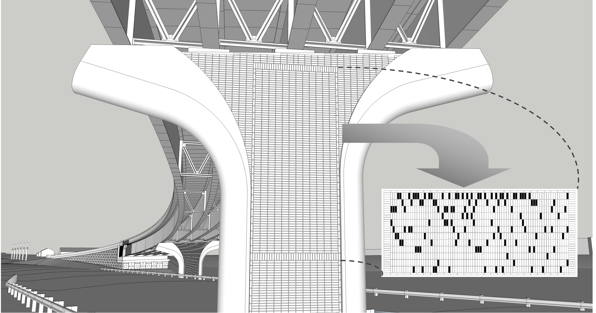
Pier "Card Section" Typical Location
