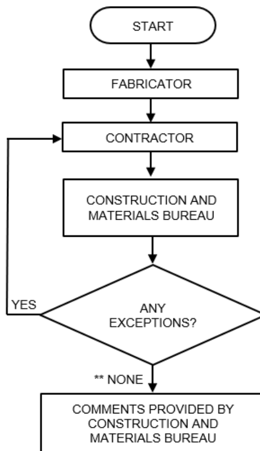
FLOW CHART OF WELD PROCEDURE REVIEWS
