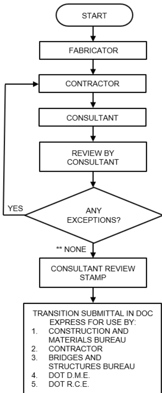
FLOW CHART OF STRUCTURE FABRICATION DRAWING REVIEWED BY CONSULTANT
