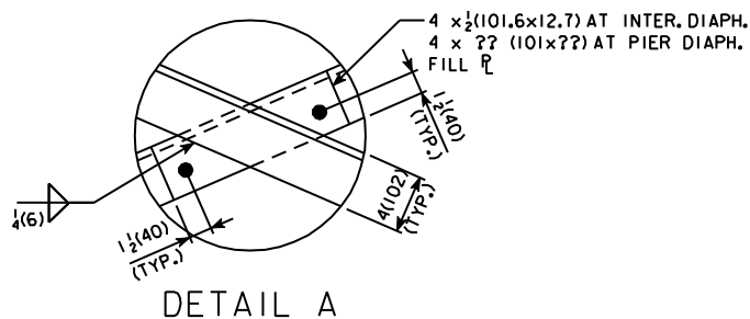
Figure 5.5.1.4.1.16-2. Alternate bolt detail at brace member crossing
