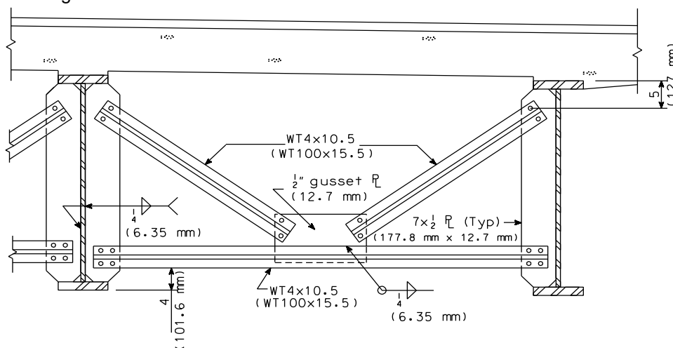
Figure 5.5.1.4.1.16-3. Alternate K-brace diaphragm for girder webs 36 inches deep or less
