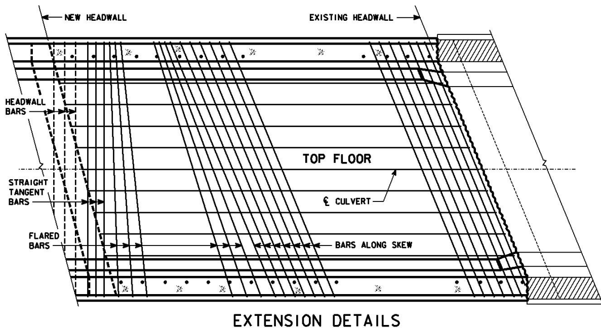
Figure 7.2.4.9.2-3. Top of floor skewed m1 bar layout
