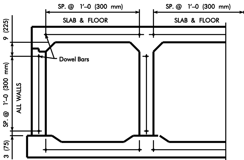
Figure 7.2.4.9.1-2. Cross section at dowels for multiple barrel extensions
