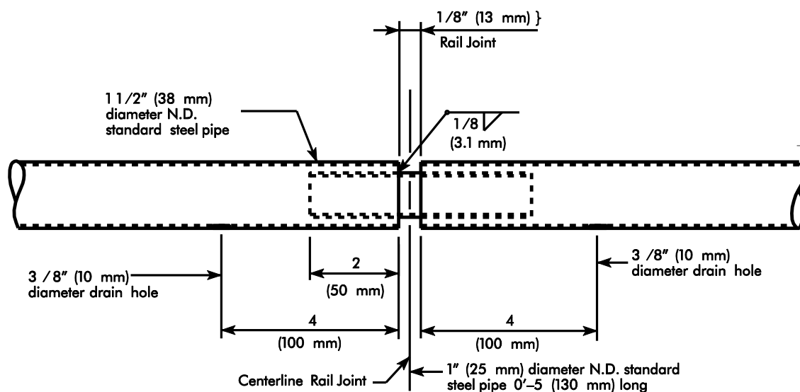
Figure 7.2.4.11.3-2. Typical urban post base plate and shim details
