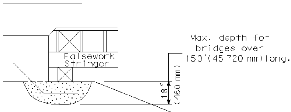
Figure 11.2.5-2. Concrete mudsill
