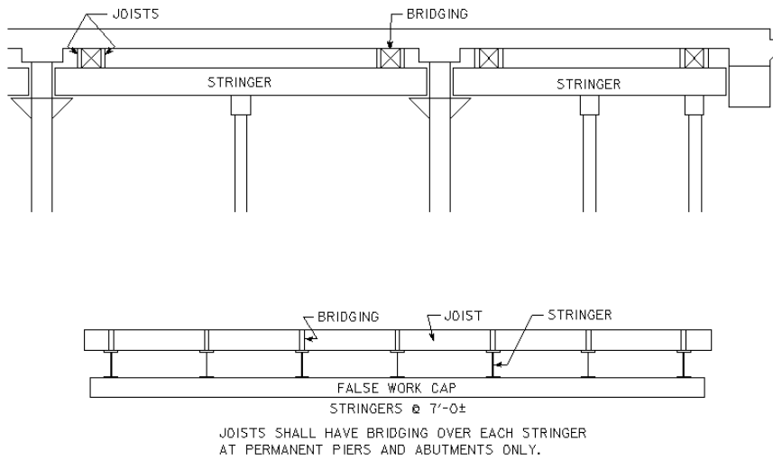
Figure 11.2.5-1. Falsework bridging
