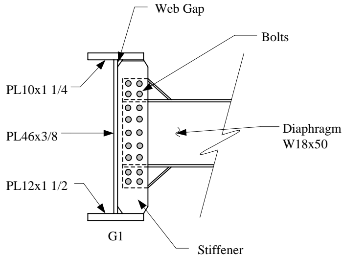
c. Diagram of a typical diaphragm/girder connection in the negative moment region of bridge 5075.5R080.
