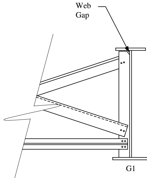
d. Diaphragm connection with web gap at stiffener clip on bridge 4048.2S017.
