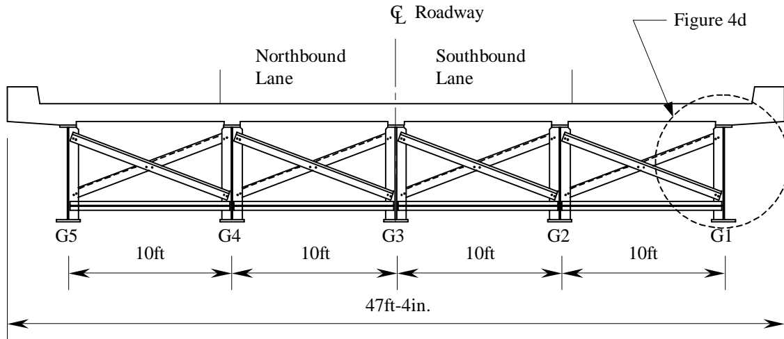
c. Cross section of bridge 4048.2S017.
