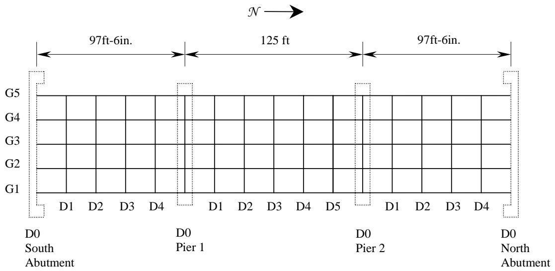
b. Plan view illustration of bridge 4048.2S017 superstructure.
