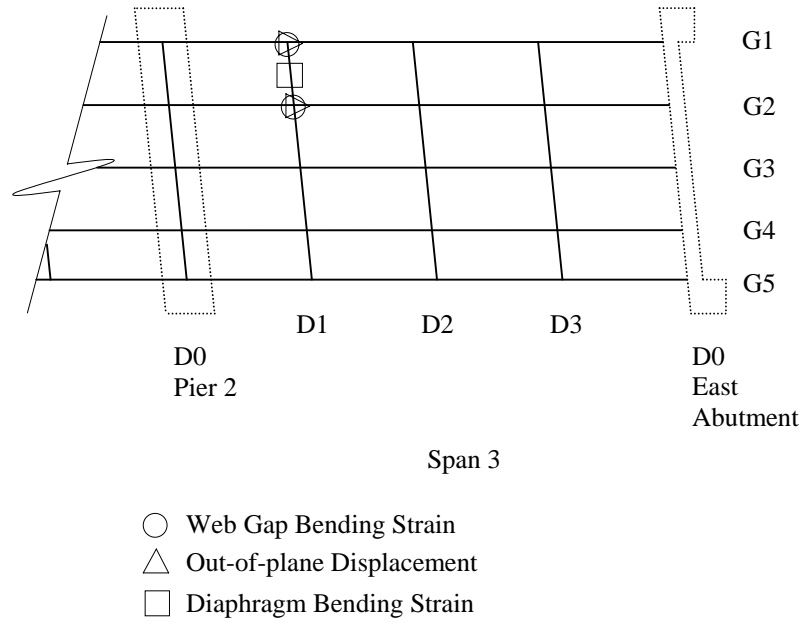
Figure 5: Typical plan view of gage placement (bridge 5075.5R080 shown).
