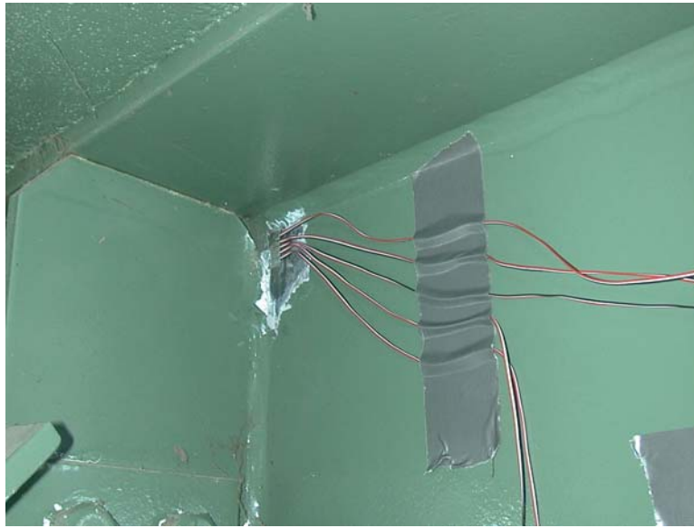
a. Typical web gap gradient instrumentation (bridge 5075.5R080 shown).
