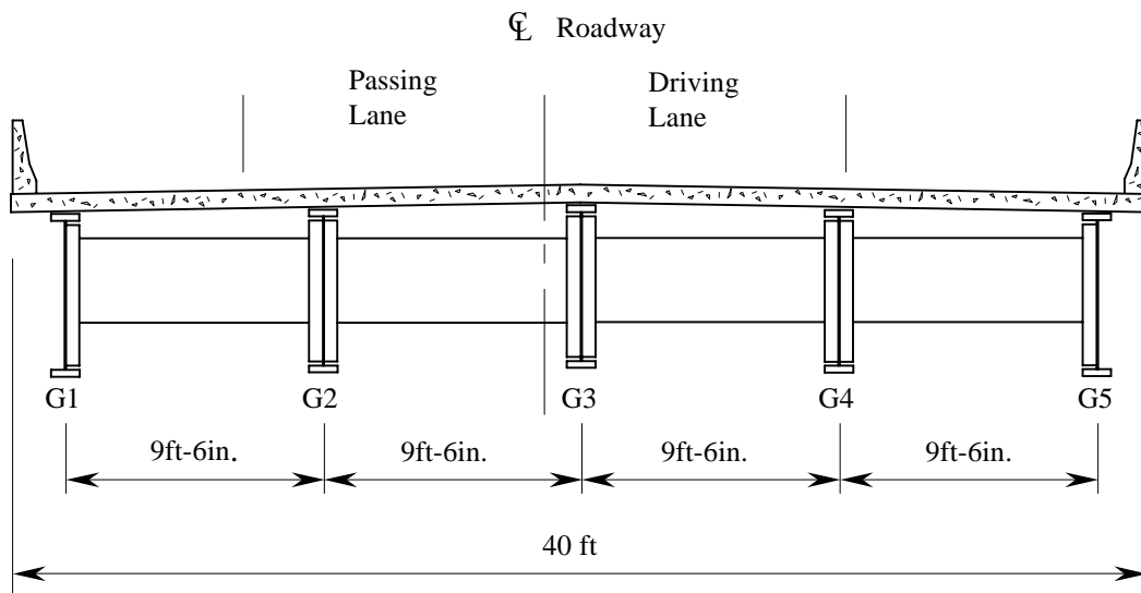
b. Cross section of bridge 2700.0R035 looking in direction of traffic.
