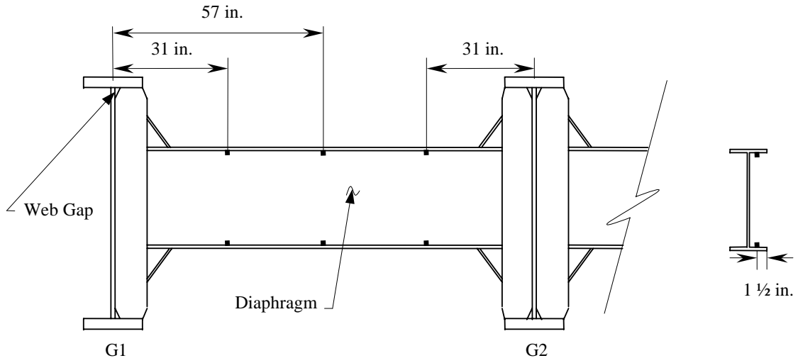
c. Typical diaphragm strain instrumentation looking east and south (bridge 5075.5R080 shown).
