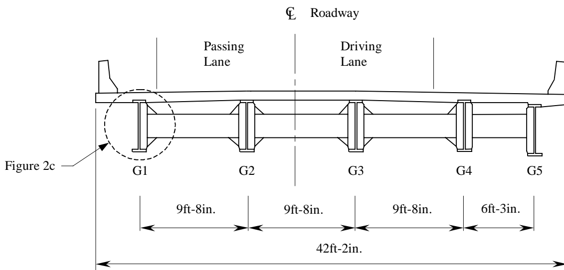
b. Bridge 5075.5R080 cross section looking toward direction of traffic.
