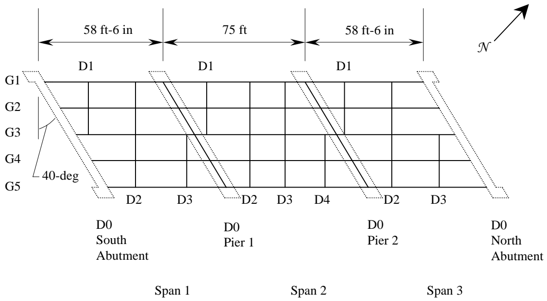
c. Plan view of bridge 2700.0R035 superstructure.
