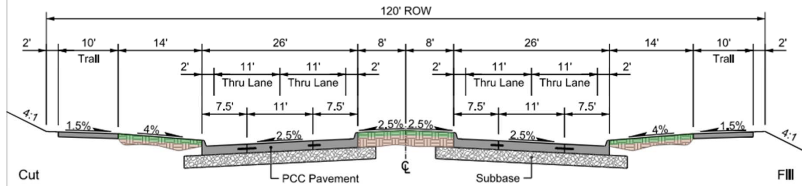
TOWER TERRACE ROAD - FUTURE 4 LANE
