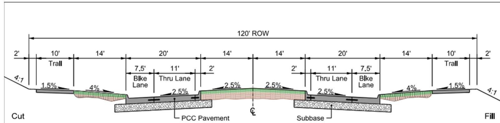
TOWER TERRACE ROAD - INITIAL BUILD - 2 LANE WITH BIKE LANES
