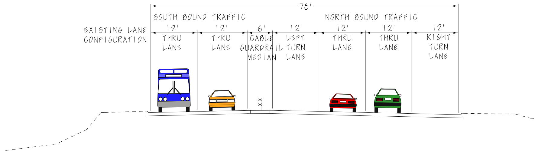
EXISTING LANE CONFIGURATION ON IA 27 / 58 SOUTH OF RIDGEWAY AVENUE
