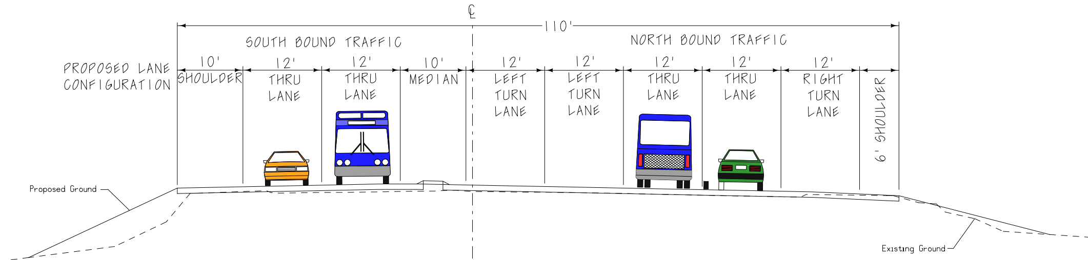
PROPOSED LANE CONFIGURATION ON IA 27 / 58 SOUTH OF RIDGEWAY AVENUE
