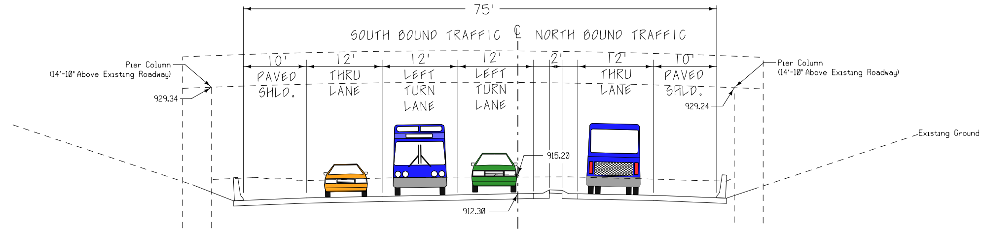
IA 27/58 CROSS SECTION UNDER US 20 BRIDGES STA. 90+75.00
