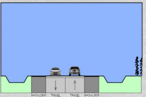
US 75 2-LANE SECTION WITH SHOULDERS
