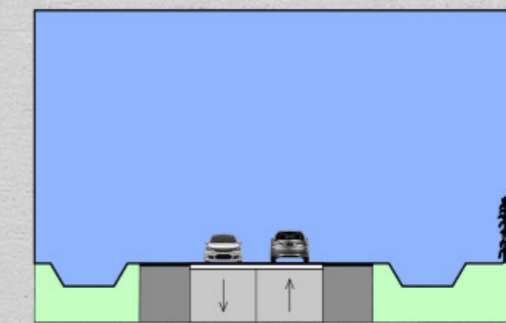
US 75 2-LANE SECTION WITH SHOULDERS
