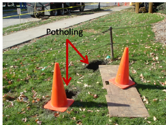
Figure 4.59. Potholing to verify position of nearby utilities
