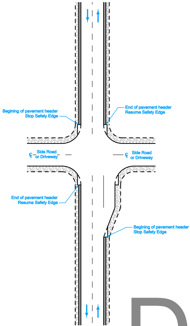
AUXILIARY LANES AND INTERSECTIONS
